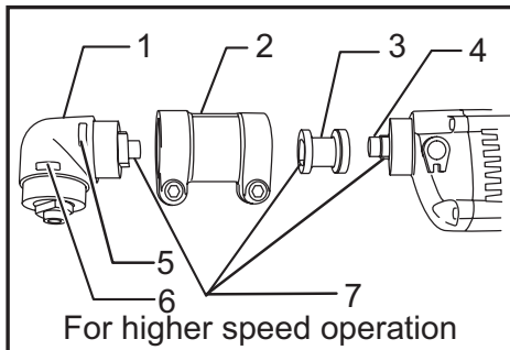
► 1. Angle housing 2. Joint 3. Socket 4. Spindle 5. Low 6. High 7. Two faces
