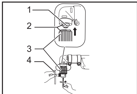
► 1. Spindle 2. Two faces 3. Drill chuck 4. Chuck key
