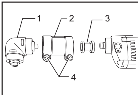
► 1. Angle housing 2. Joint 3. Socket 4. Bolt
